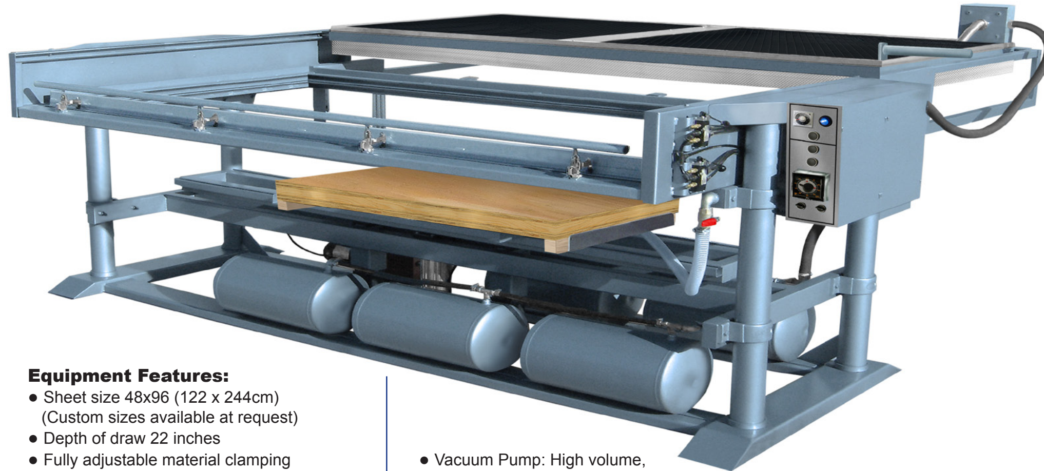
Option: Vacuum Former with Overhead Assist
